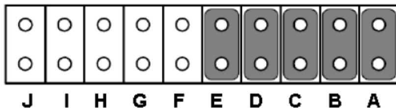
Figure 2.11 RS-232 Jumper Setting
